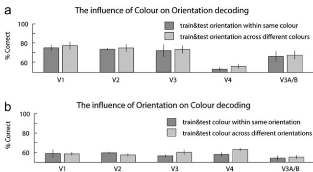
Figure 4. Invariance of orientation coding with respect to color and vice versa. (a) The classifier was trained to discriminate responses to orientation stimuli presented in one color, and then tested on responses to orientation presented in the same or different color. Classifier performance was not affected when training and test stimuli were different colors. (b) Color discrimination: the classifier was trained to discriminate responses to red or green stimuli in one orientation and then tested on responses to color stimuli presented in the same or opposite orientation. Classifier performance was not affected when training and test stimuli had different orientations. Error bars: SE across 5 subjects.
