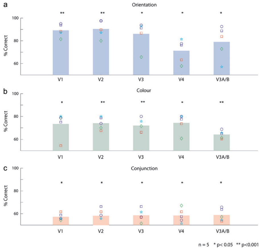
Figure 2. Discrimination performance of a linear classifier (SVM) at orientation, color, and double-conjunction stimuli. (a) Decoding of orientation (CW vs. CCW) was significantly above chance (chance = 50%) in every ROI, averaged across 5 subjects. (b) Decoding of color (red vs. green) was also significant in each area (c) decoding of double-conjunction stimuli (GCW&RCCW vs RCW&GCCW) reached significance in all areas. Symbols: single subject-decoding performances ( n = 5 subjects).
